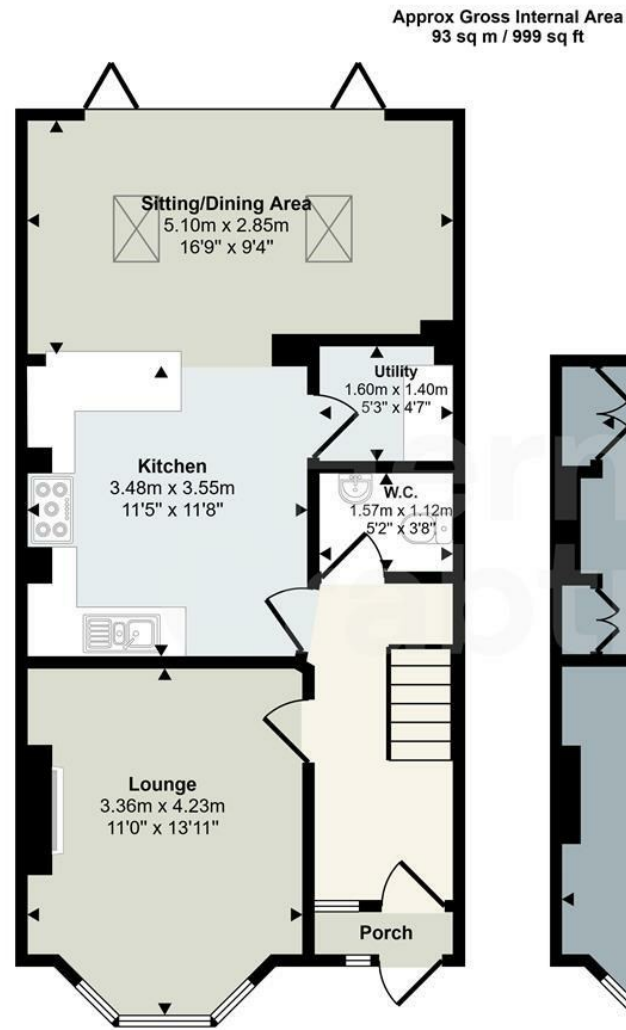
Ground Floor Approx 54 sq m / 582 sq ft
